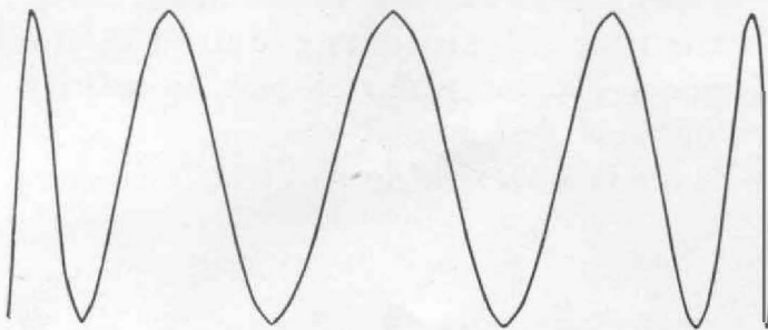
FIGURE 4. Characteristic Lissajou figure from applying a voltage E_h across horizontal plates having exactly \frac{1}{10} th the frequency and twice the amplitude of the voltage E_v applied to the vertical pair. Note that the pattern near the center is an approximation to the true shape of E_v since the spot velocity due to E_h is nearly constant in this region. The "back trace" coincides with the forward sweep for this particular phase difference ( 90^\circ )
