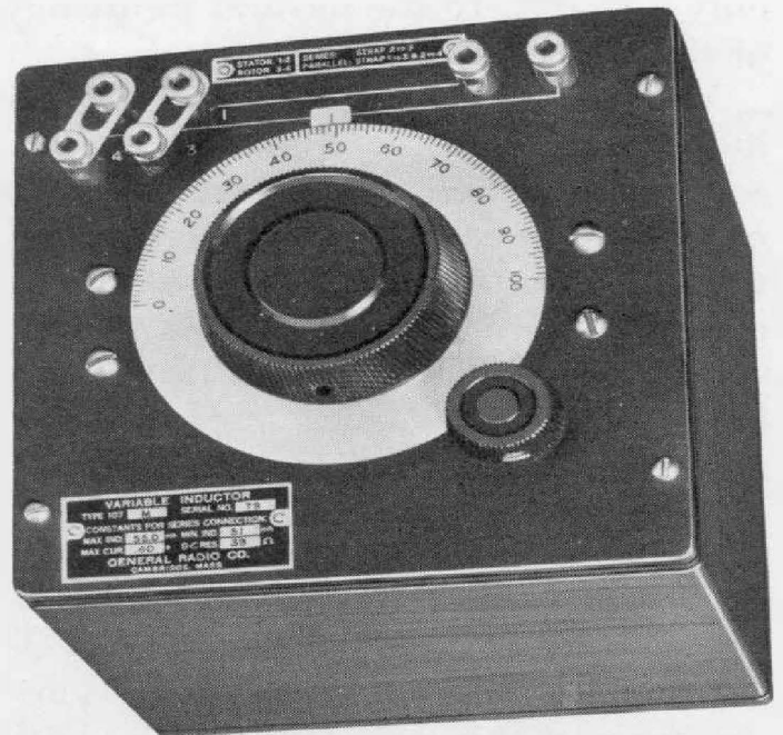
One of the new TYPE 107-M Variable Inductors with rotor and stator connected in parallel
