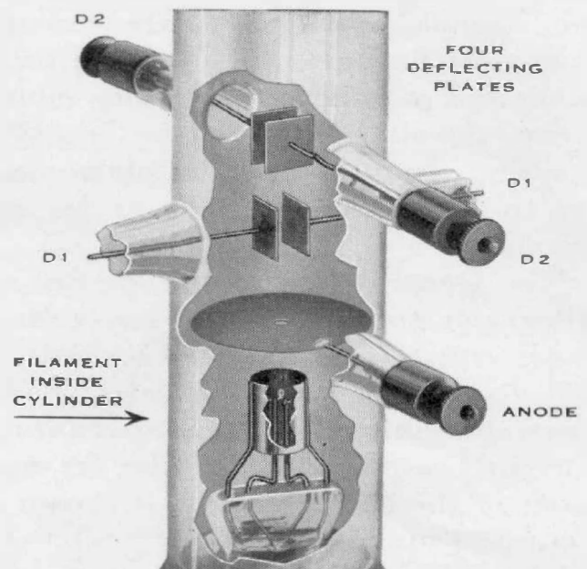
FIGURE 2. Electrode structure of the oscillograph tube. The negatively charged cylinder concentrates the electrons emitted by the filament so that practically all pass through the small hole in the anode. The beam passes between each pair of deflecting plates
