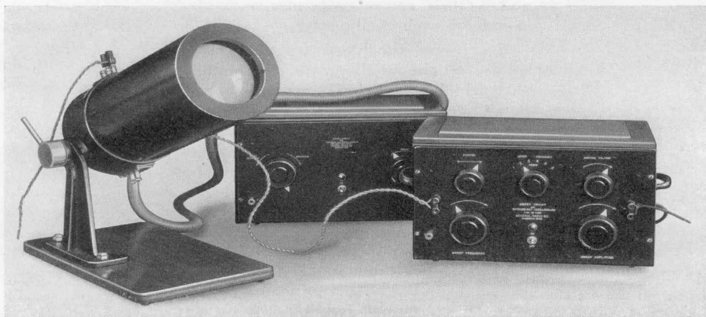
FIGURE 7. The TYPE 506-A Sweep Circuit is shown at the right of the mounted oscillograph tube and its a-c operated power supply equipment
