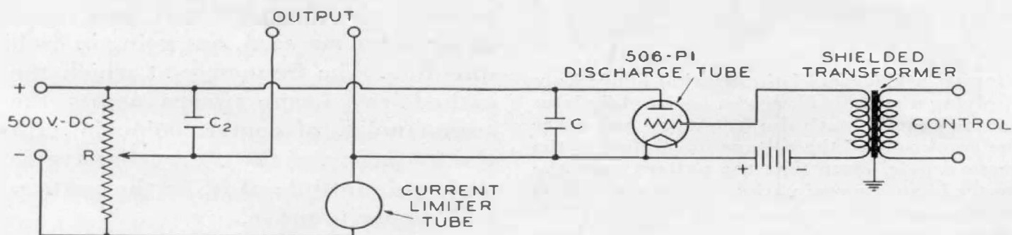
FIGURE 6. Schematic diagram of the TYPE 506-A Sweep Circuit
