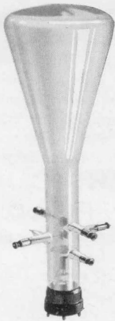
FIGURE 1. The General Radio cathode-ray oscillograph tube. The inside of the glass at the large end is coated with a fluorescent substance on which the moving beam of electrons traces patterns
